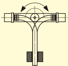
Reversed bending test with swinging according to PMA spec.9.21-4425 & IEC EN 61386 (搖擺反向彎曲強度測試)
