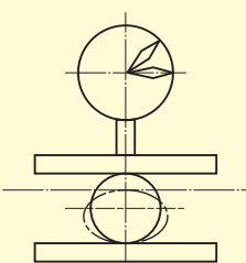
Peak load test according to PMA spec.9.21-4320 & IEC EN 61386 (抗壓強度測試)
