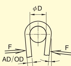
Cold bending test according to PMA spec.9.21-4380 (低溫彎曲強度測試)
