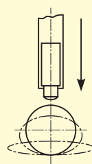
Impact test according to PMA spec. 9.21-4330 & IEC EN 61386 (硬度測試)
